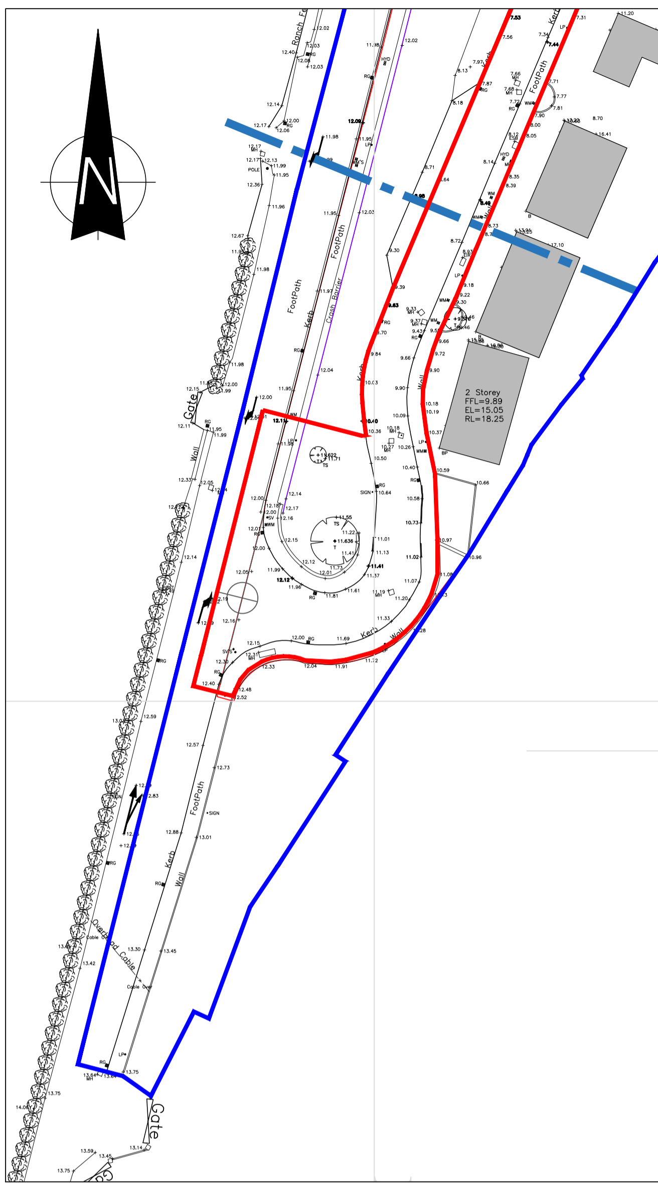
Site Survey - Entrance Scale 1:500
